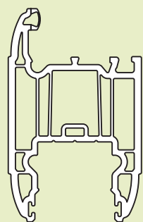
LPD082 Sash
