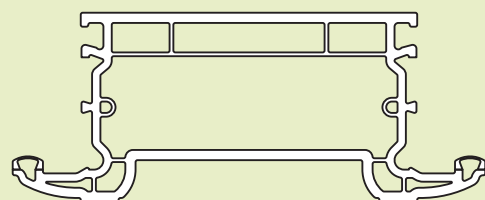
LPD084 Midrail
