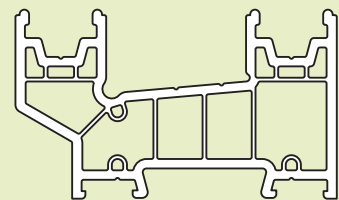
LPD081 Outer Frame
